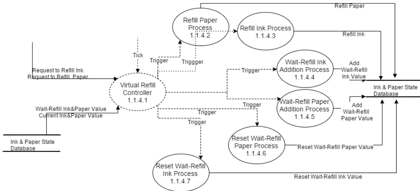
DFD Level 4 on Virtual Refill Process
